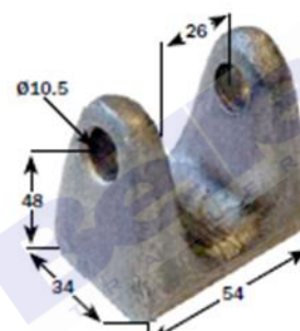
TAILBOARD FORKET - WELD ON (SELF COLOUR)
