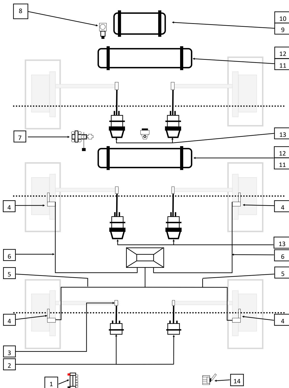
TYPICAL TRAILER BRAKE LAYOUT
